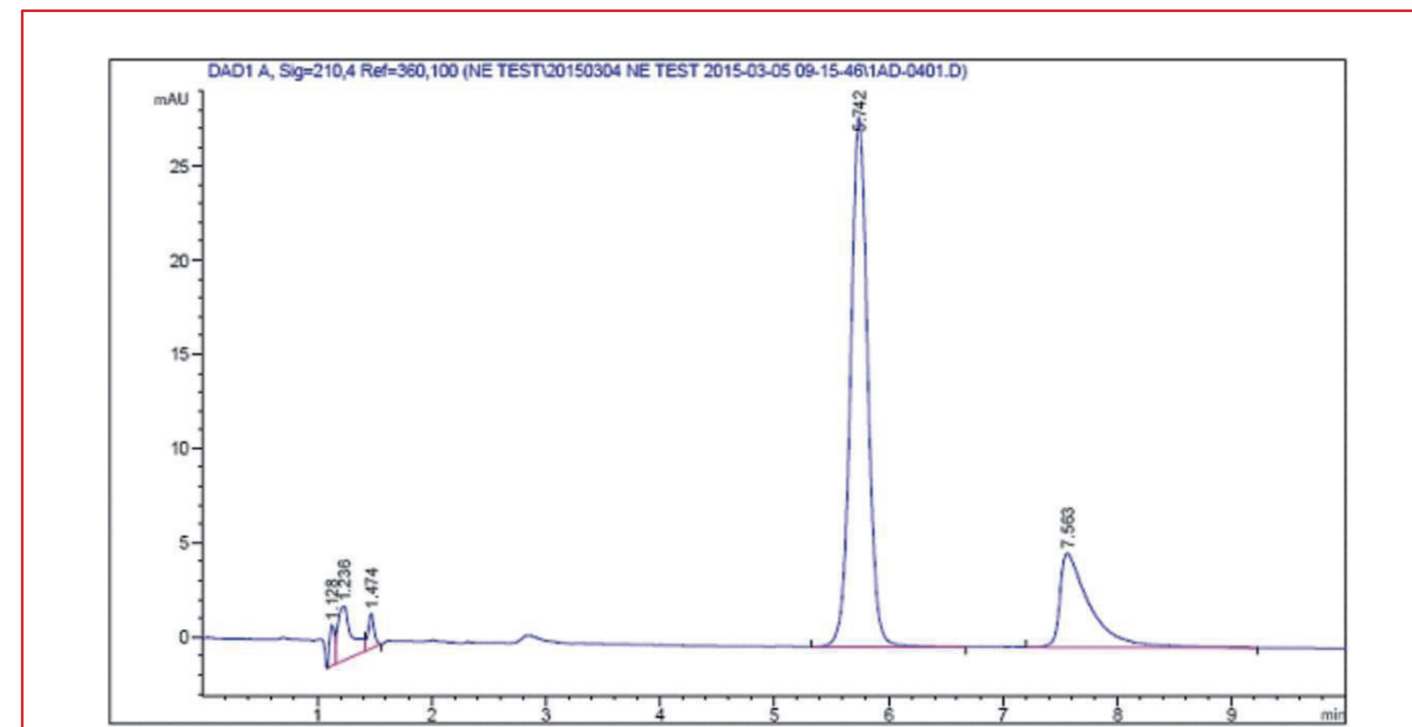
Figure 1. Chromatogram of norephedrine (NE) extracted from Recatol capsules
